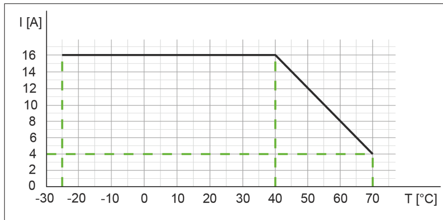
III. 3: Derating sensor current I_{US} / actuator current I_{UA}
